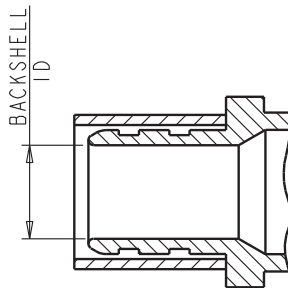
SECTION A-A -003 ACCESSORY
